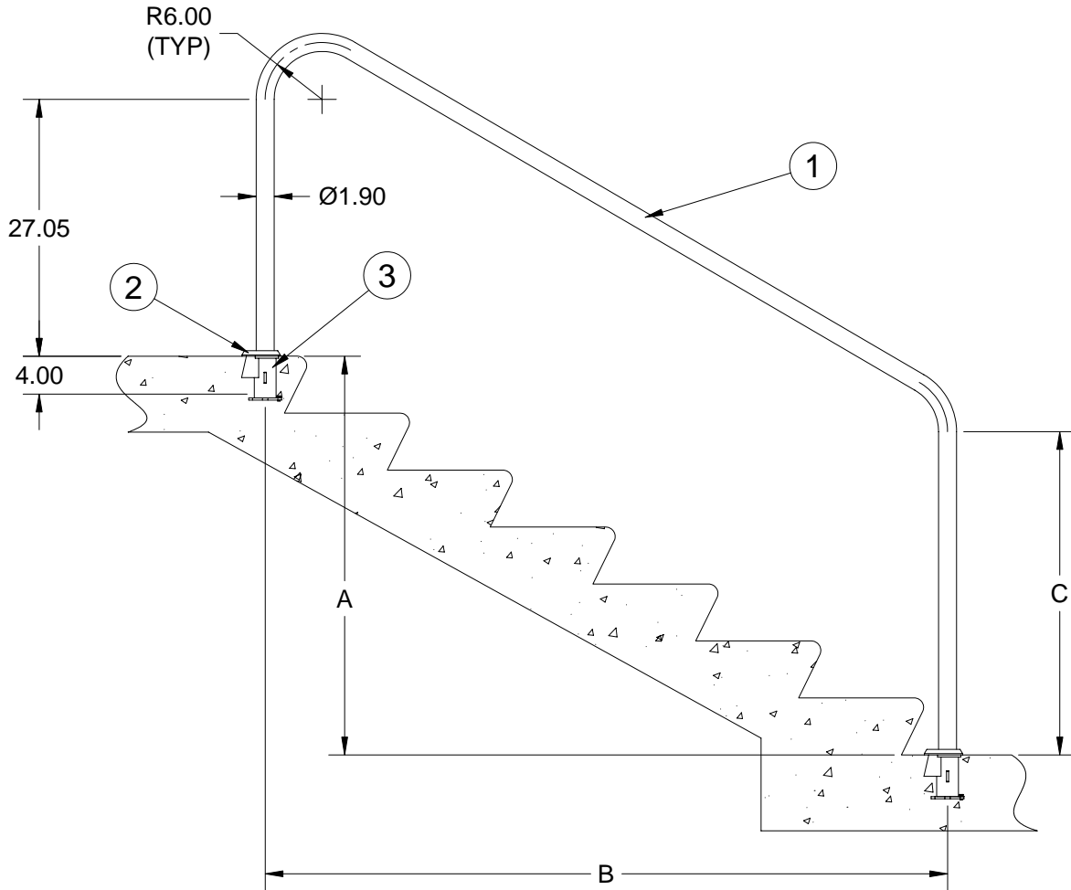
SIDE VIEW
