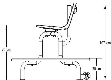
76 cm O-Series Lifeguard Chair
