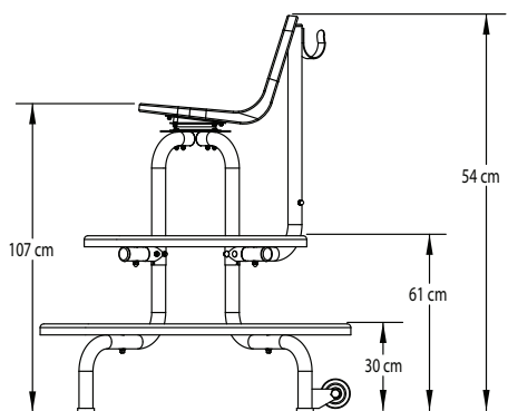
107 cm O-Series Lifeguard Chair
