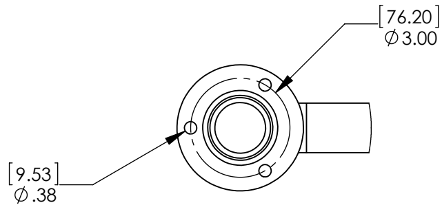
DETAIL B SCALE 1 : 4
